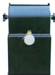
Econo-Safe #AGKC0001 Constructed of 10 gauge steel 11-1/2" W x 10-1/4" D x 19" H Handle and Locks project 1-3/4"
